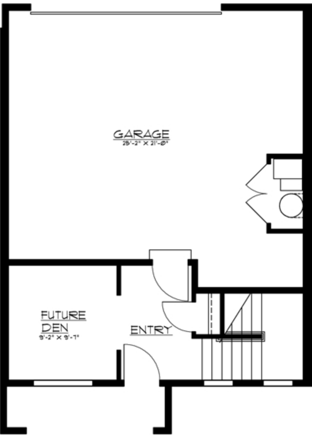
UNIT "D" FIRST FLOOR PLAN
