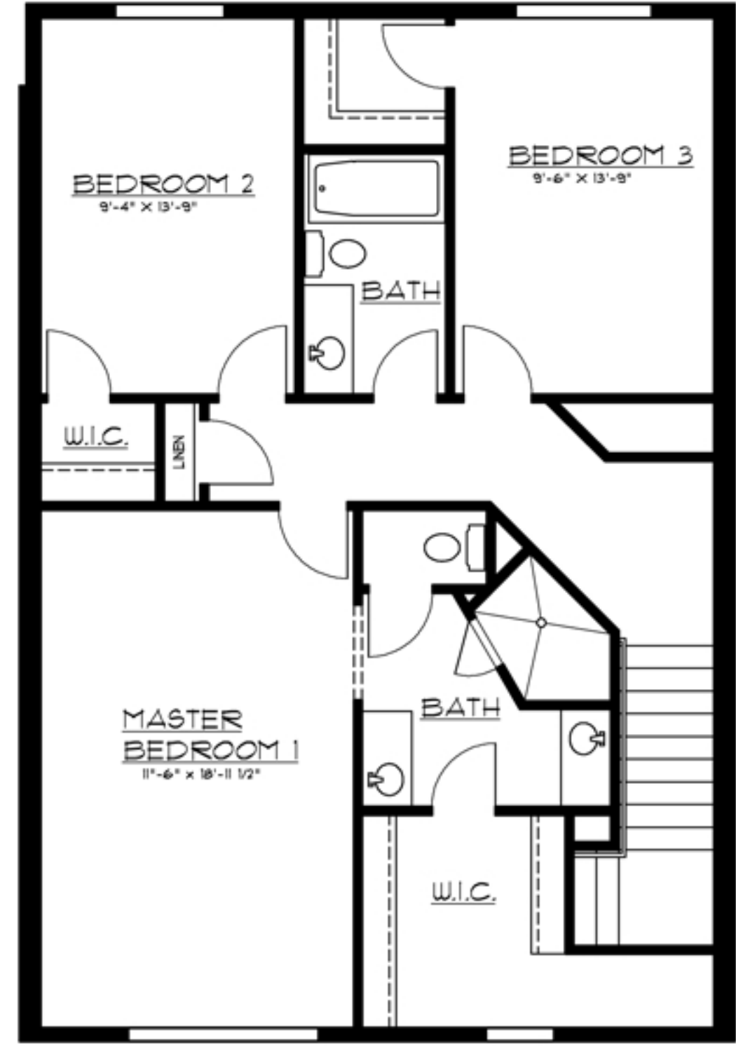
UNIT "D" THIRD FLOOR PLAN
