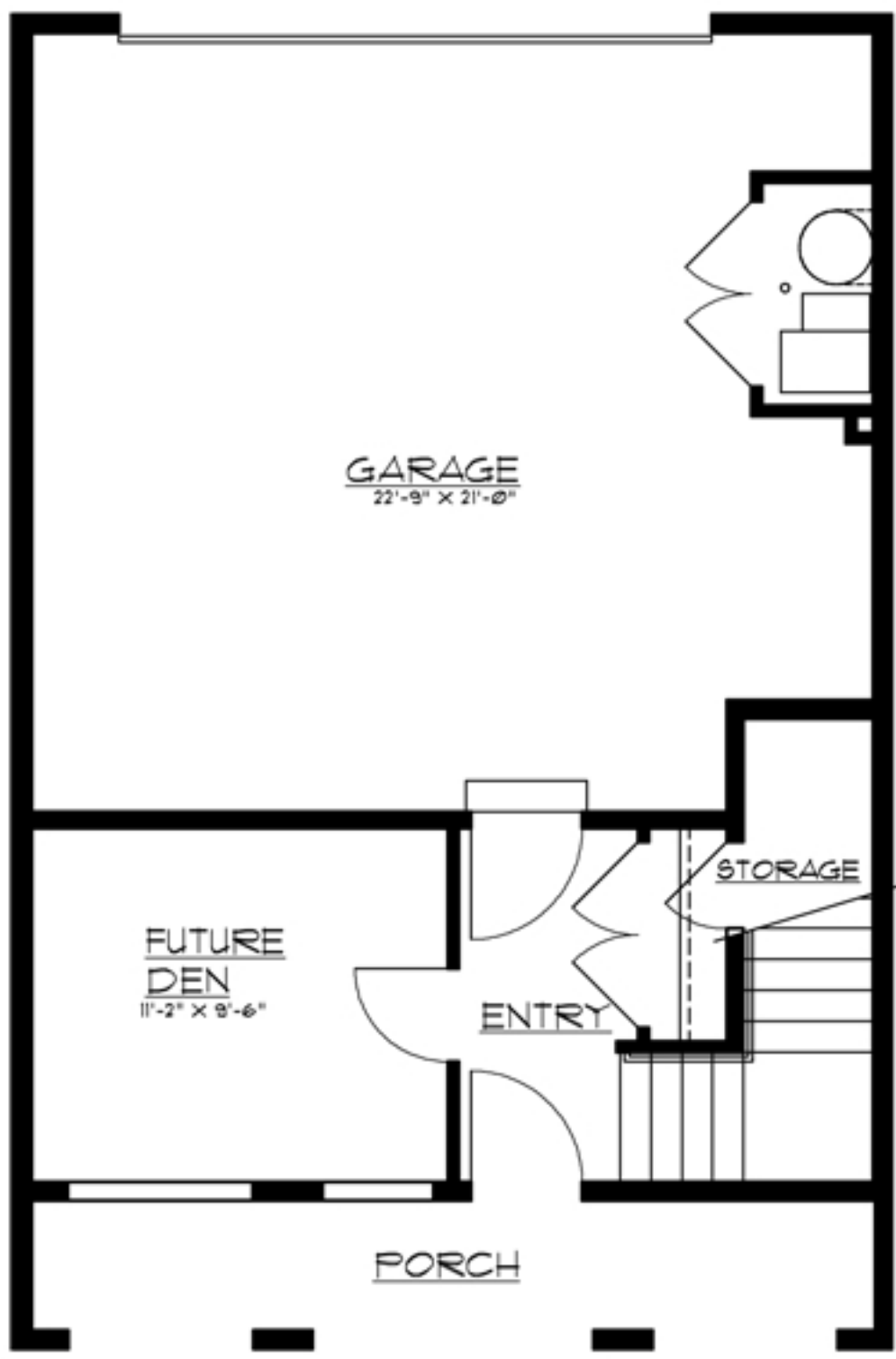
UNIT "C" FIRST FLOOR PLAN
